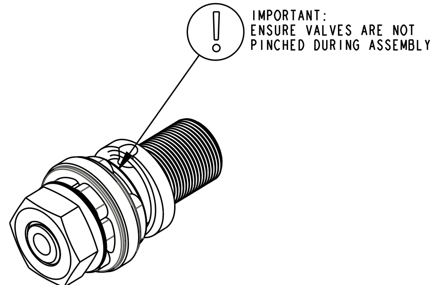
DETAIL A SCALE 2.000
