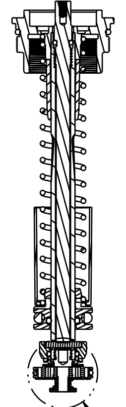
SECTION A-A SEE DETAIL Z
