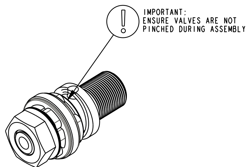
DETAIL A
