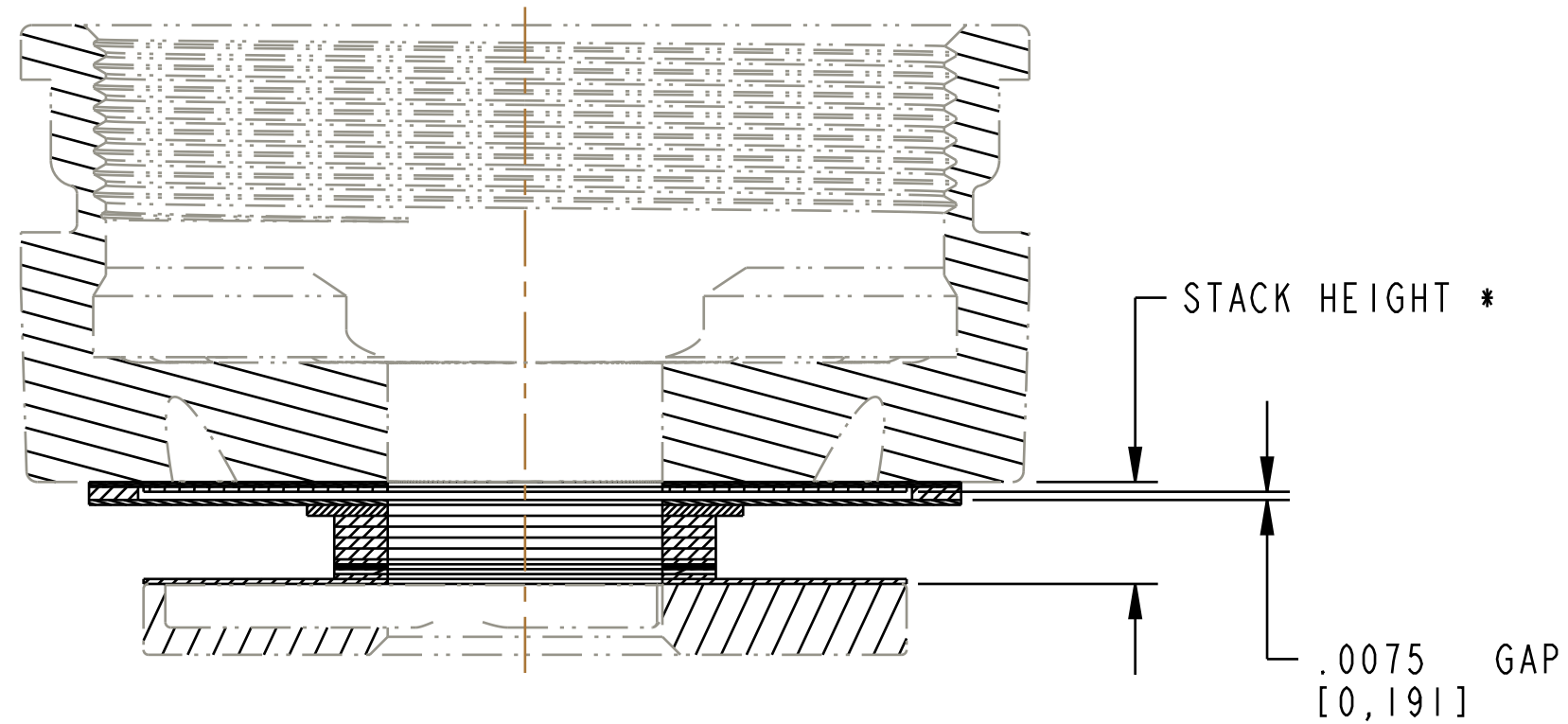
SECTION A-A SCALE 6:1
