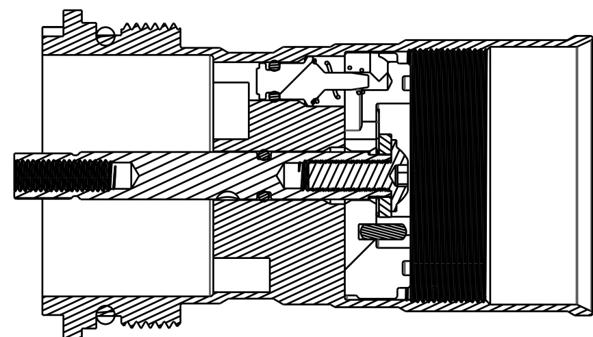
SECTION C-C
